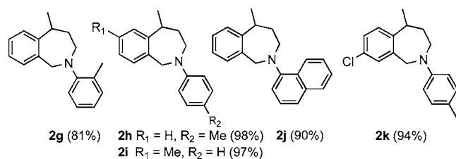
Figure 1. Other 2-benzazepines prepared by the three-component one-pot approach. All reactions were performed by using 0.50 mmol each of aldehyde and aniline, 7.5 mol % of I , 2.5 mL of toluene, under 800 psi CO/H 2 (7:1), at 120 °C, for 48 h. Isolated yields are shown.
